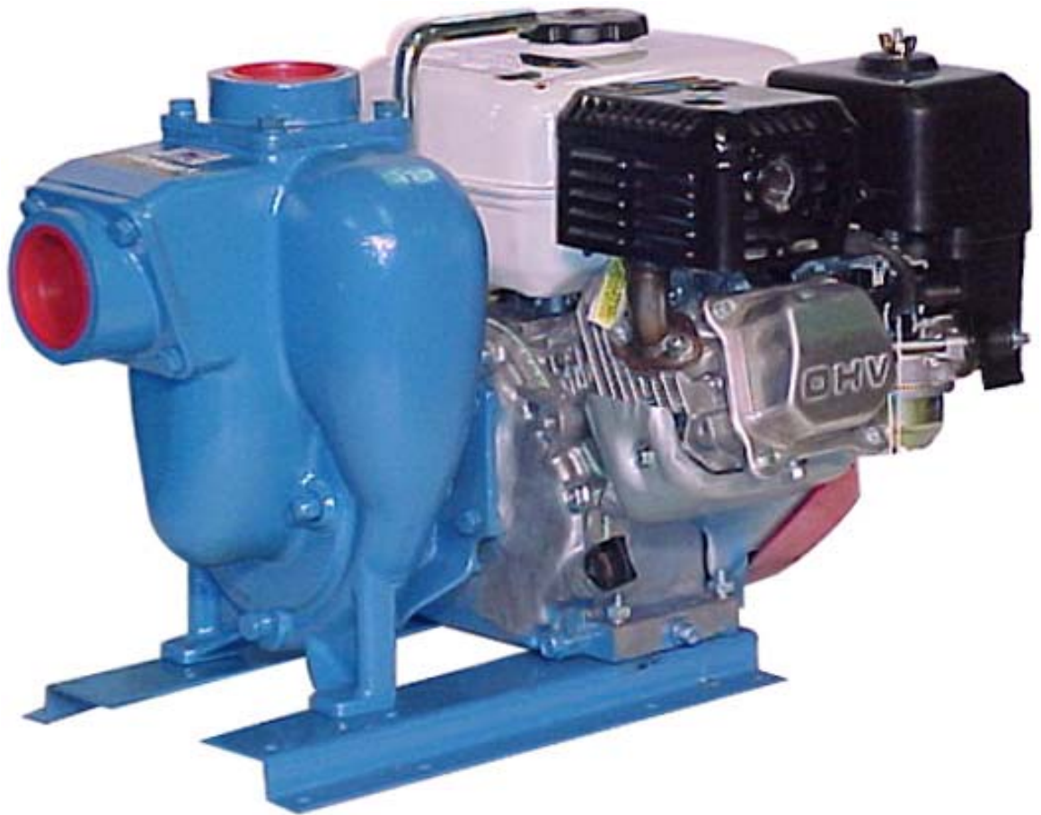
Flomax 8 2" Fertilizer Pump & Engine Combo Units
